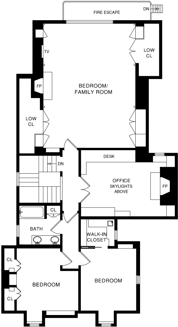
FOURTH LEVEL
