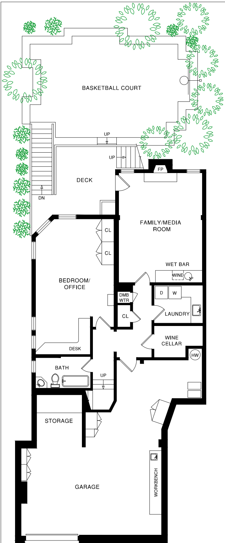
LOWER LEVEL
